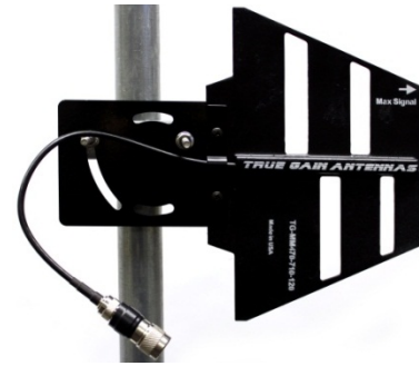
TG-MM470-710-120 475 MHz / Vertical
